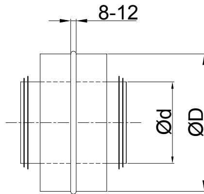
isolation 10 mm
